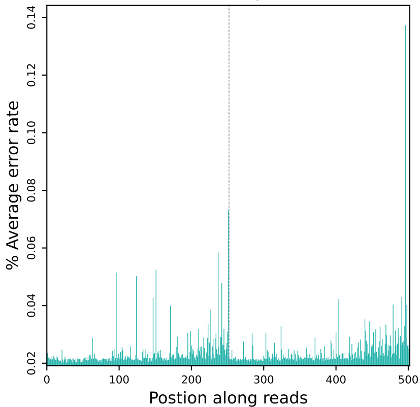
Error rate distribution along reads (R10317)
